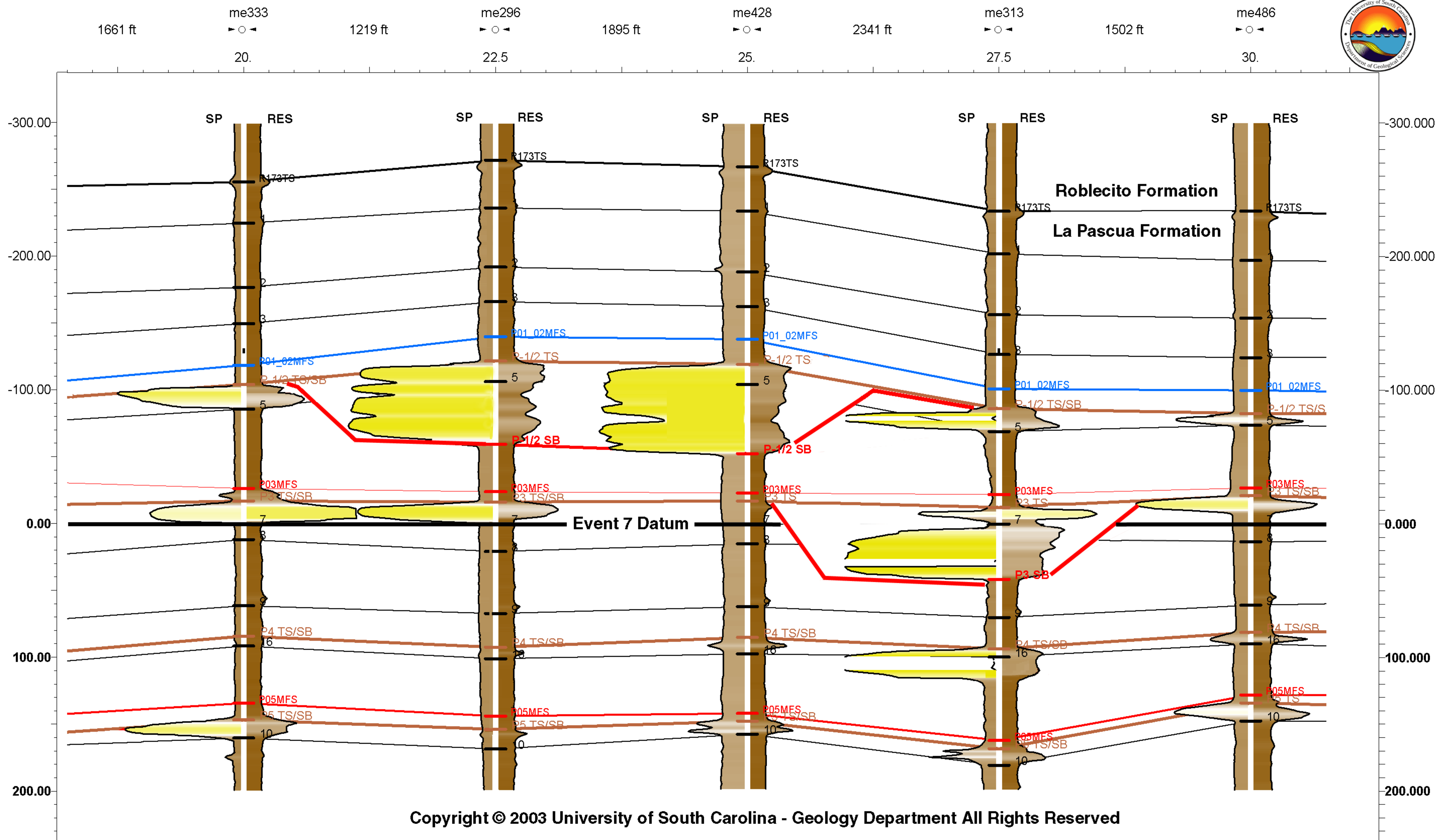
Interpreted Well Log Section (SP & Resistivity Logs) - 5 Wells of the Northern Strike Line, Las Mercedes Field, Guarico Sub Basin, NE Venezuela Oligocene Upper Pascua Formation (Final 3 Sequences). Flattened on "Event" 7 shale kick datum; at base is the P5 SB and at top is contact between La Pascua and Roblecito Formations (Reistroeffe 2001). Depths in feet relative to the "Event" 7 datum. Section Assembled and interpreted by P. Lake, C. G. St.C. Kendall and J. Reistroeffe - July 2003. For academic and educational puposes only.
